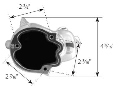
3 Hole bolt pattern
